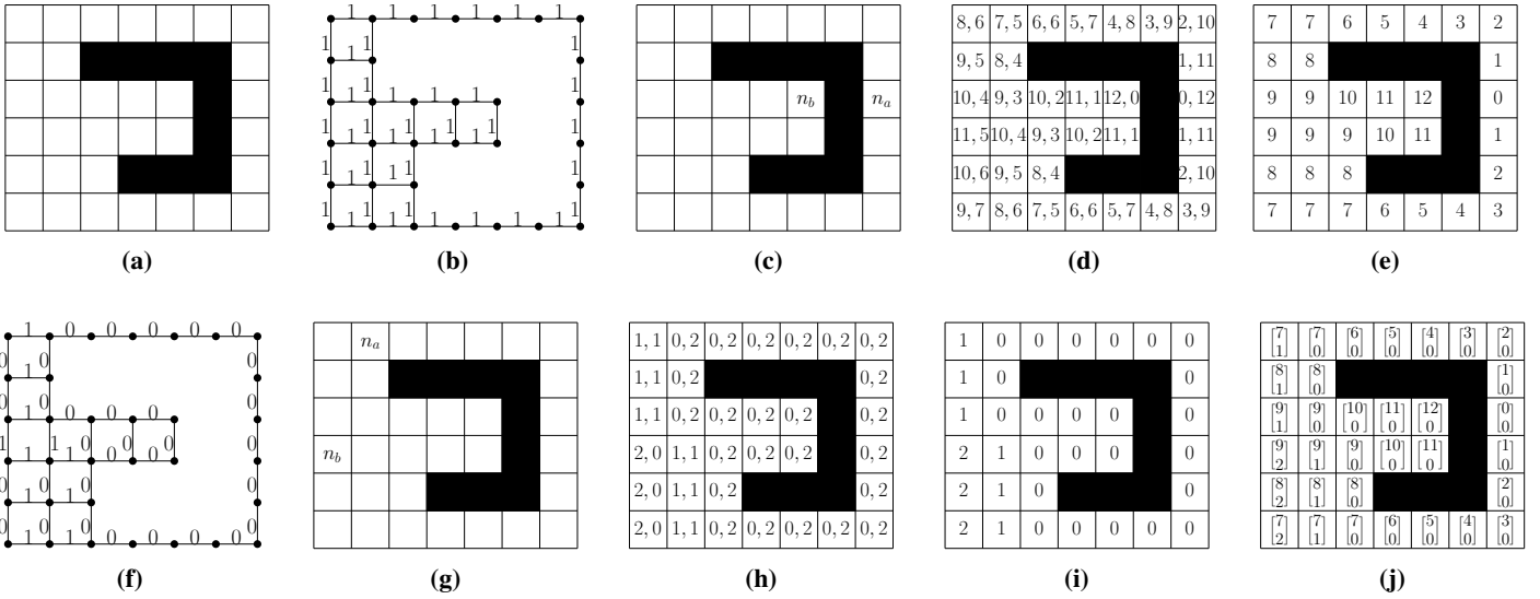
Figure 3: Illustrates the working of FastMap. (a) shows a 4-neighbor gridworld with obstacles in black. (b) shows the graphical representation of (a) with the original unit weights on the edges. (c) shows the identified farthest pair of nodes. (d) shows two numbers in each cell representing the distances from n_a and n_b , respectively. (e) shows the first coordinate embedding for each cell. (f) shows new edge weights for the next iteration. (g), (h) and (i) correspond to (c), (d) and (e), respectively, in the second iteration. (j) shows the produced 2D embedding.
