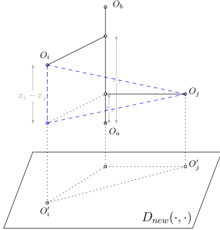
Figure 2: Shows a geometric conceptualization of the recursive step in FastMap. In particular, D_{new}(O'_i, O'_j)^2 = D(O_i, O_j)^2 - (x_i - x_j)^2 .
