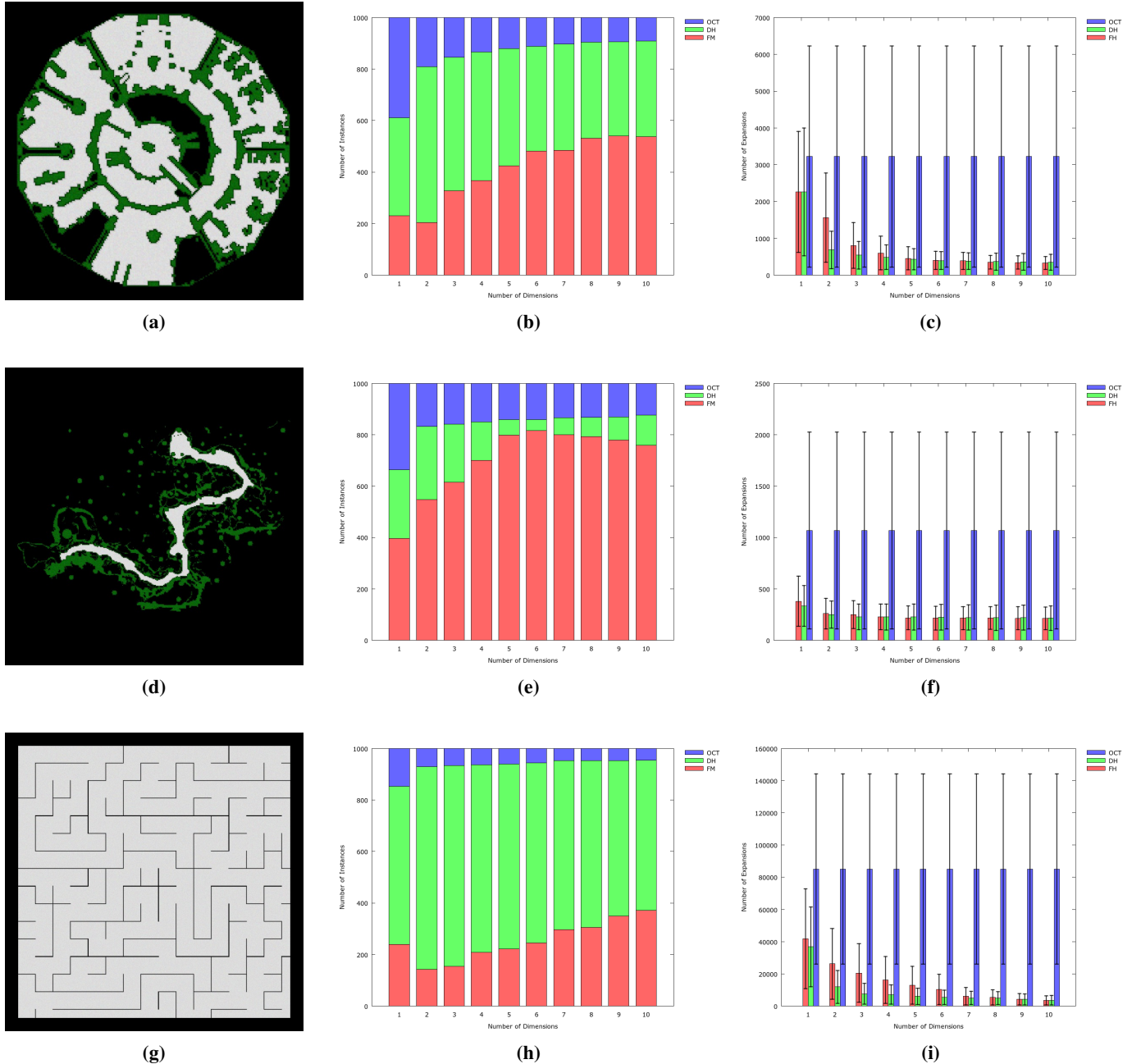
Figure 4: Shows empirical results on 3 maps from Bioware's Dragon Age: Origins. (a) is map 'lak503d' containing 17,953 nodes and 33,781 edges; (d) is map 'brc300d' containing 5,214 nodes and 9,687 edges; and (g) is map 'maze512-32-0' containing 253,840 nodes and 499,377 edges. In (b), the x-axis shows the number of dimensions for the FastMap heuristic (or the number of pivots for the Differential heuristic). The y-axis shows the number of instances (out of 1,000) on which each technique expanded the least number of nodes. Each instance has randomly chosen start and goal nodes. (c) shows the median number of expanded nodes across all instances. Vertical error bars indicate the MADs. The figures in the second and third rows follow the same order. In the legends, "FM" denotes the FastMap heuristic, "DH" denotes the Differential heuristic and "OCT" denotes the Octile heuristic.
