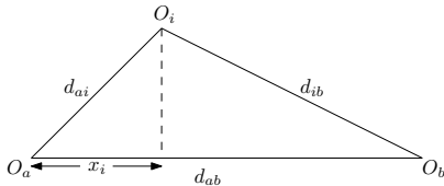
Figure 1: The three sides of a triangle define its entire geometry. In particular, x_i = (d_{ai}^2 + d_{ab}^2 - d_{ib}^2)/(2d_{ab}) .
